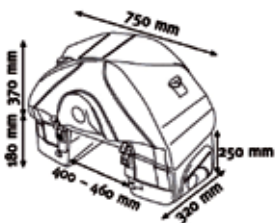
Speedpack Wide
