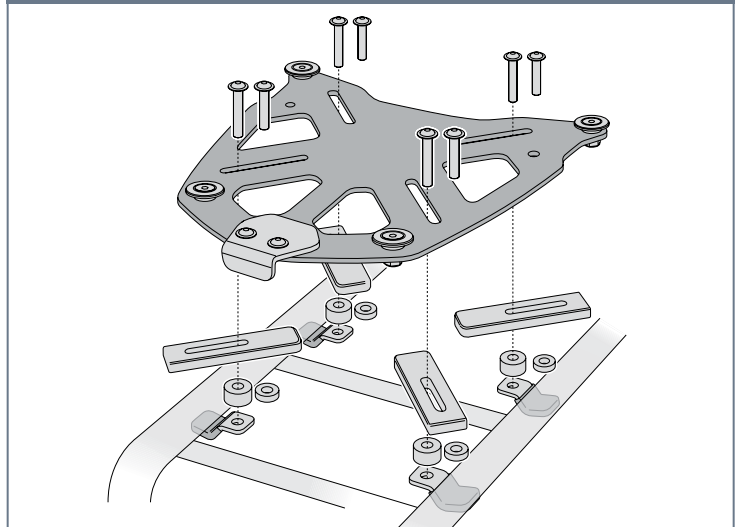
Schematic of TraX Universal Adapter Plate
