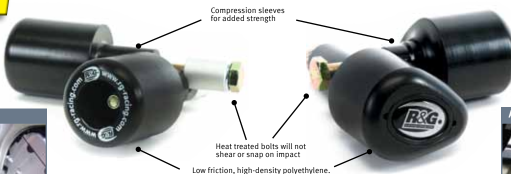
Classic Slider
